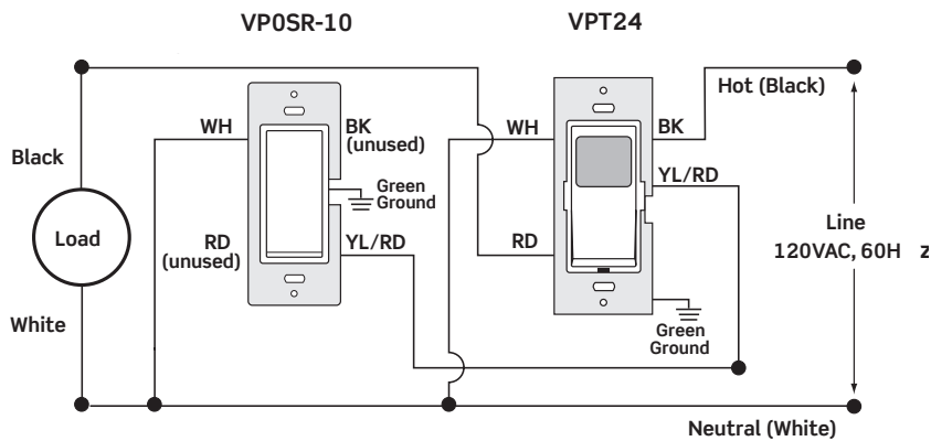
3-Way with Switch Companion, no LED (up to Nine VP0SR-10 can be used)
