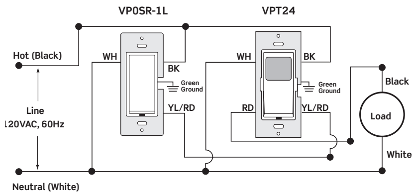
3-Way with Switch Companion (up to Four VP0SR-1L can be used)
