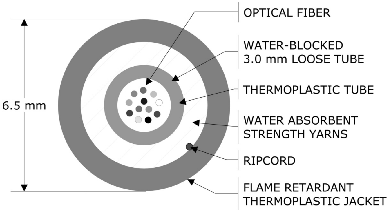
LTR012 Cross-section
